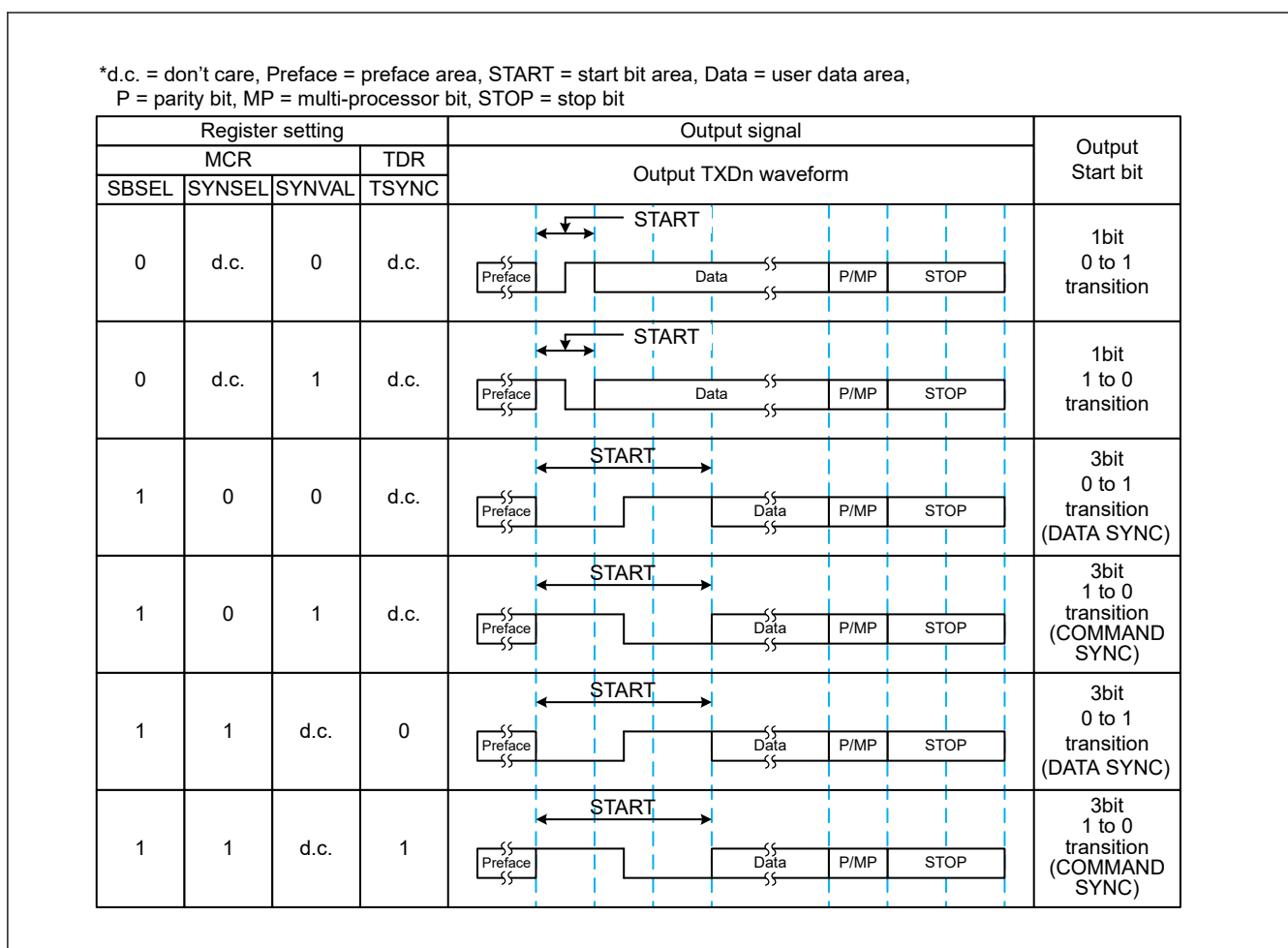
Figure 38.48 Settings Related to and Format of the Start Bit Area at Transmission
