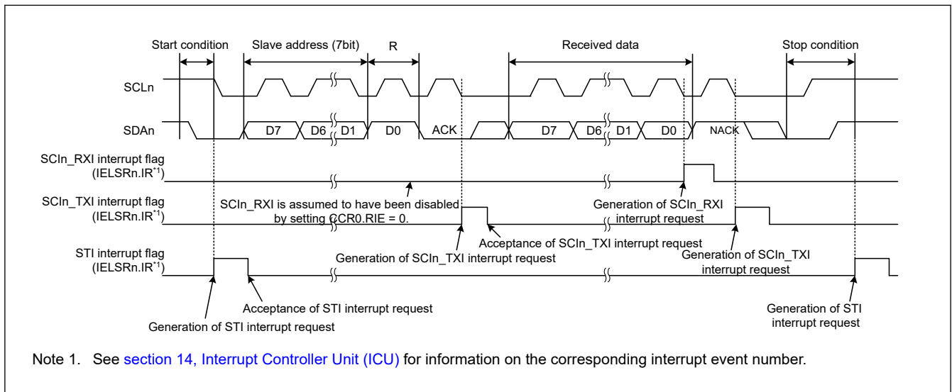
Figure 38.94 Example operations for master reception in simple IIC mode with 7-bit slave addresses, transmission interrupts, and reception interrupts (ICR.IICINTM = 1)
