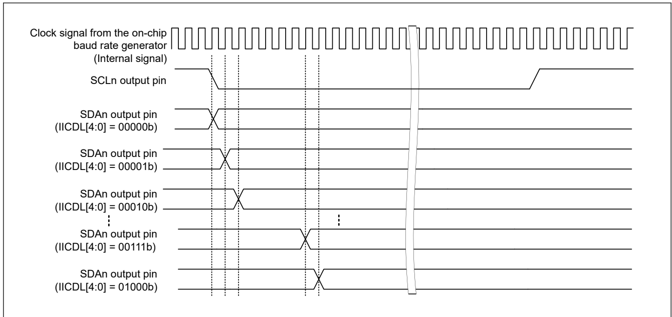
Figure 38.90 Timing of delays in SDAn output
