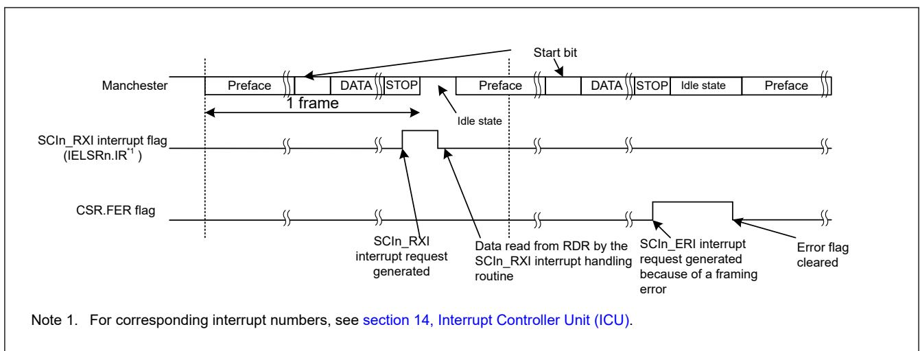
Figure 38.56 Example of Operation for Serial Data Reception in Manchester mode (with a Preface)
