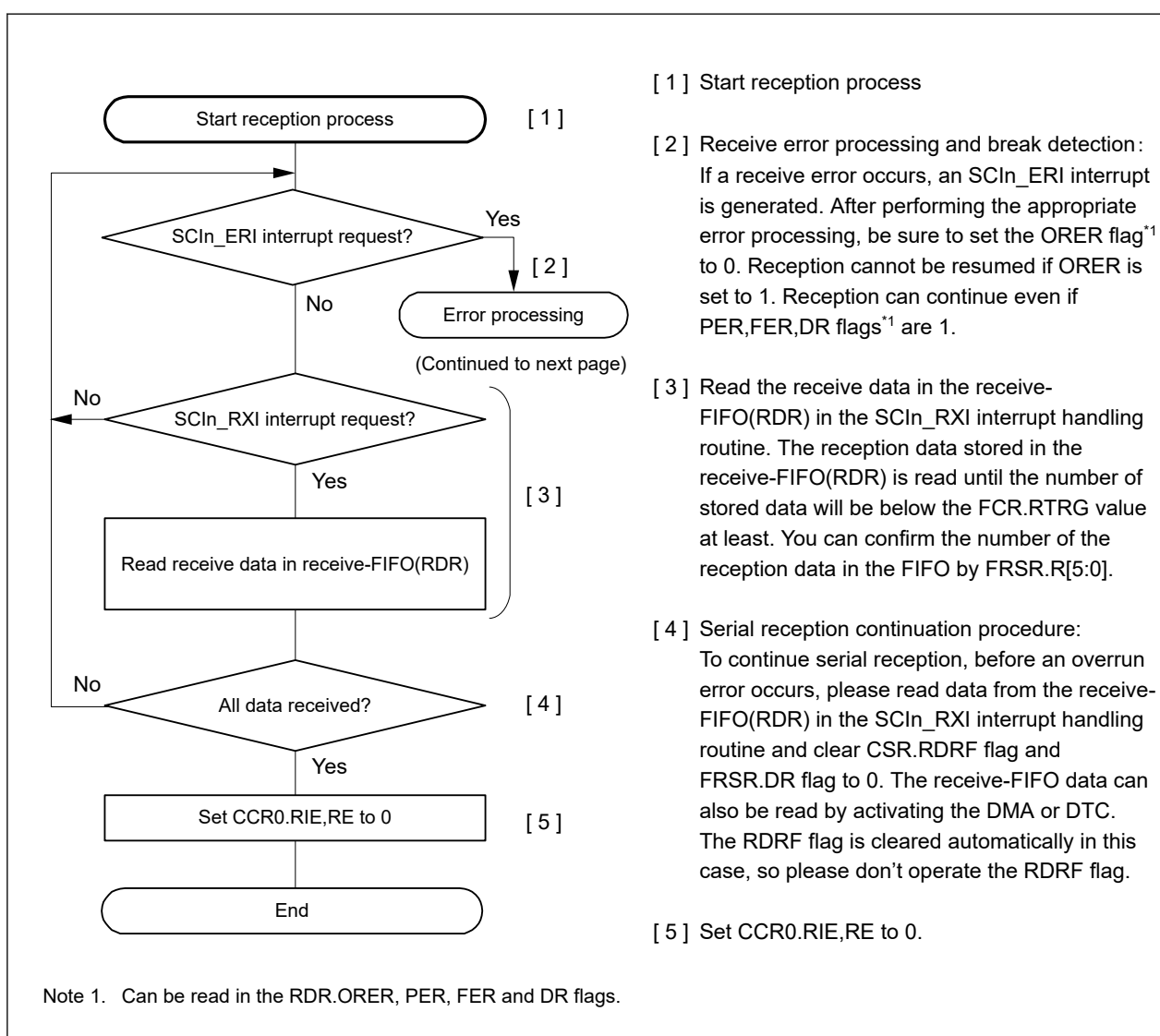
Figure 38.24 Example flow of serial reception in Asynchronous mode with FIFO selected and Address Matching Enabled (1)
