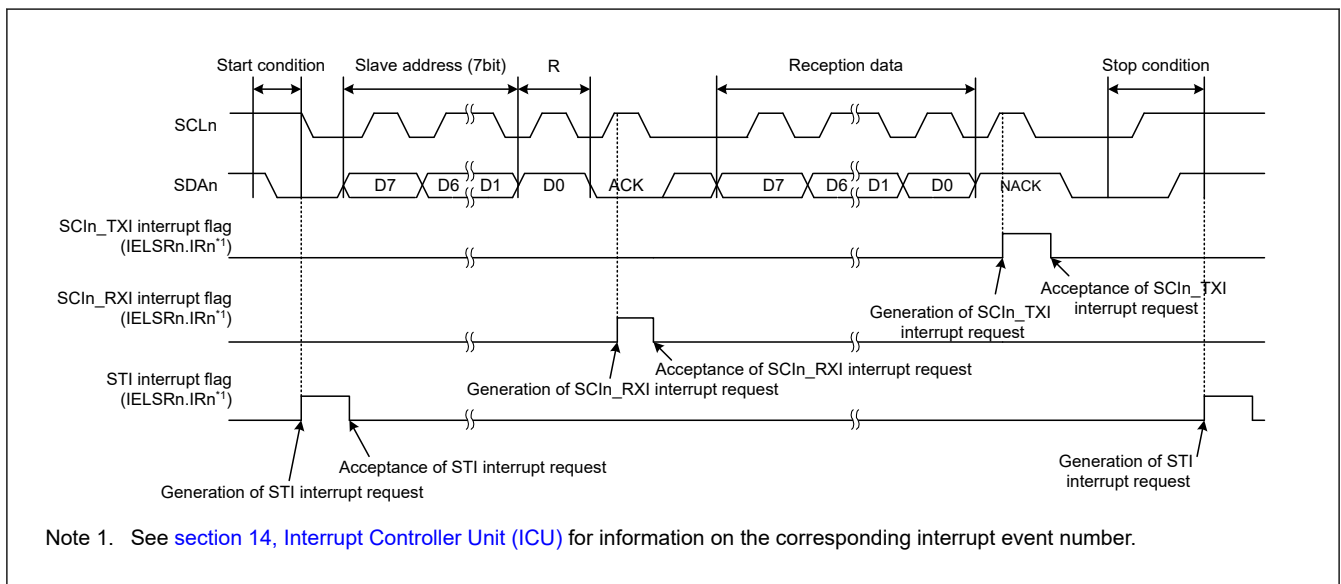
Figure 38.95 Example of Operations for Master Reception in Simple IIC Mode (7bit Slave address, ACK and NACK interrupt in use (ICR.IICINTM = 0))
